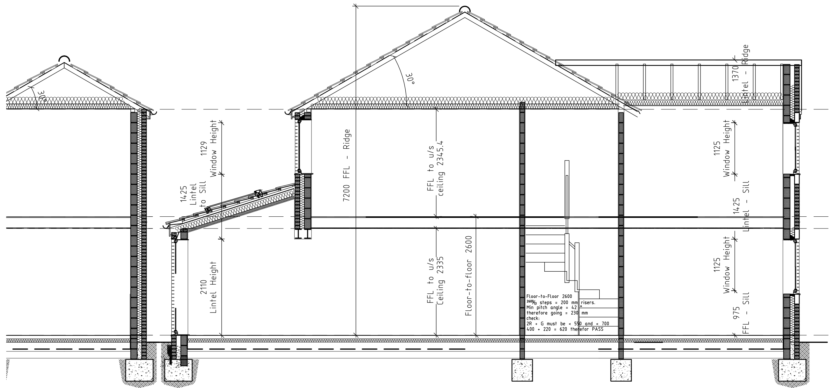
POSED (TYPICAL) SS SECTION: NT PORTION
