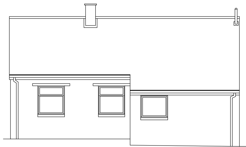
EAST ELEVATION 1:100
