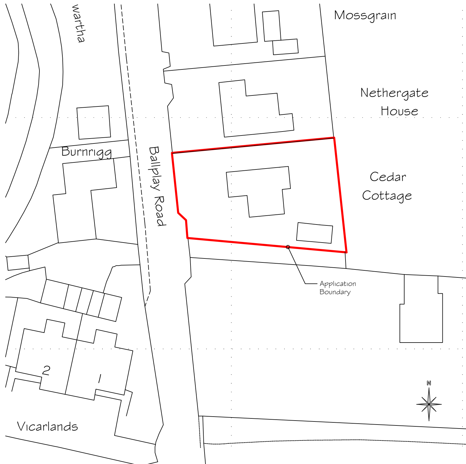
BLOCK PLAN 1:500
