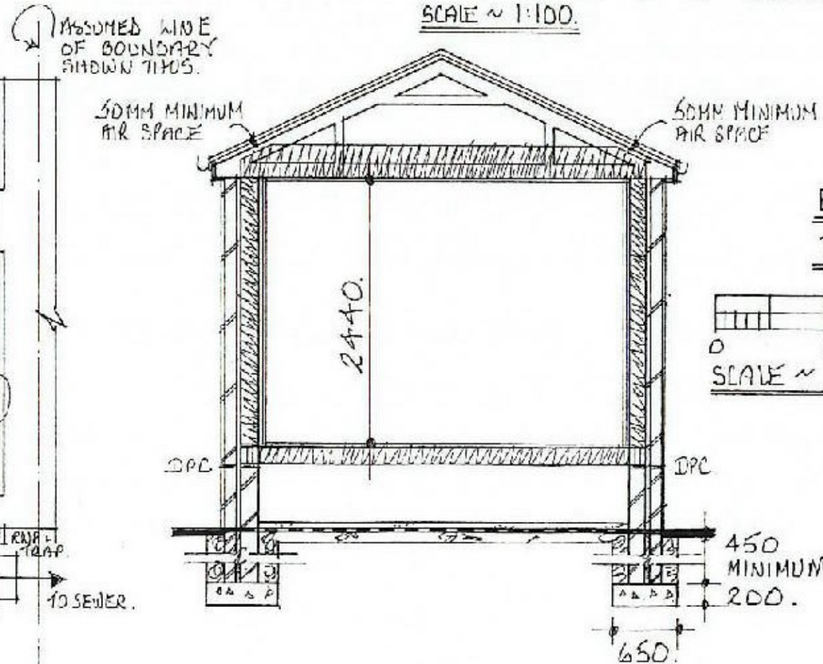
PROPOSED SECTION A - A.
