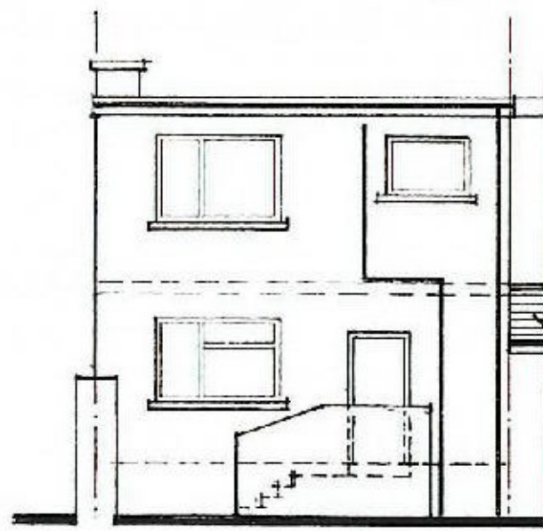
EXISTING N. W. ELEVATION.
