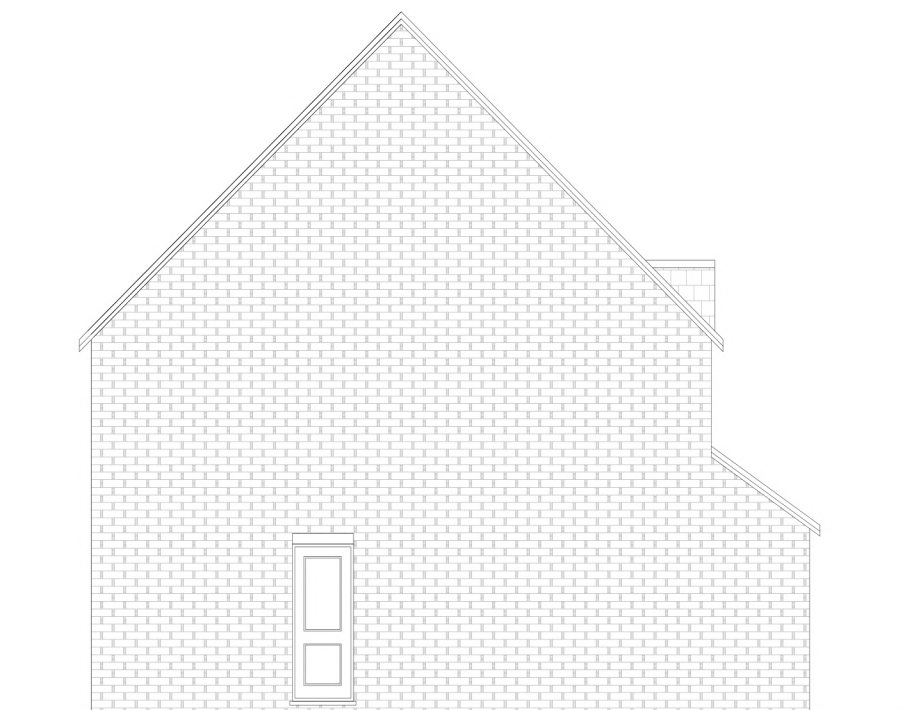
Left Elevation
