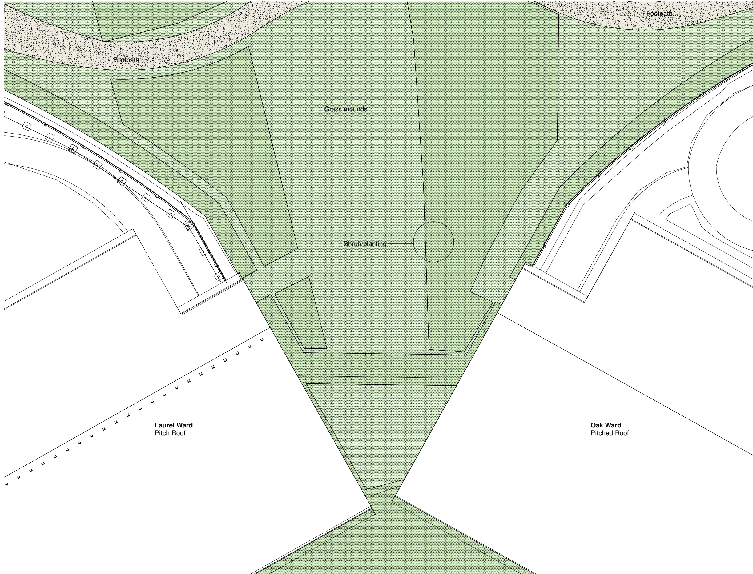
1 CC_CC-R1-0001_Existing Roof Plan 1 : 100
