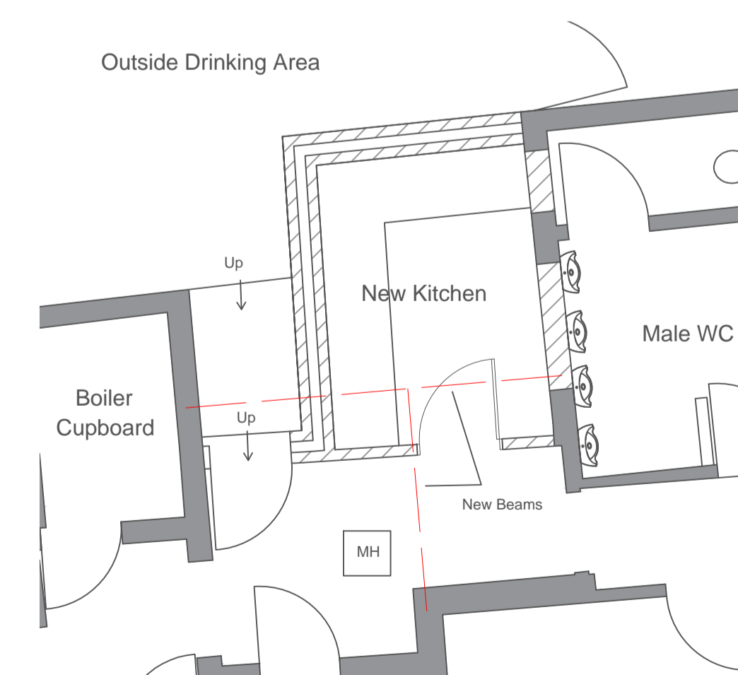
Proposed Part Plan 1:50
