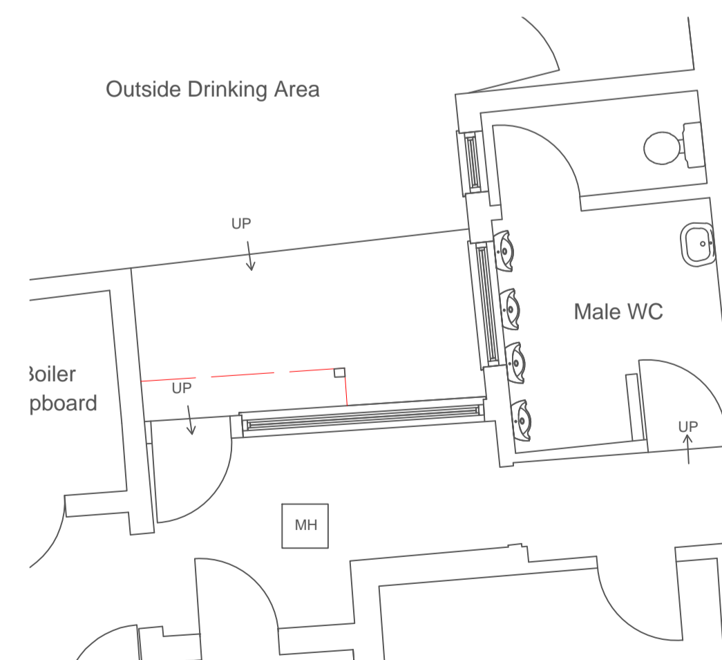
Existing Part Plan 1:50
