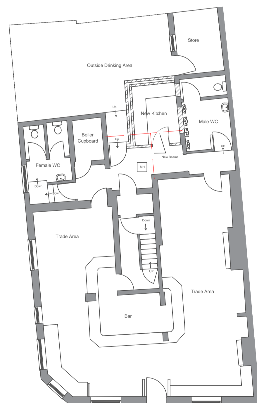
Proposed Floor Plans 1:100
