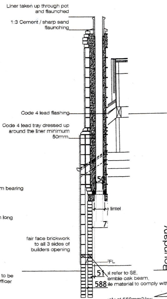
Section B-B
