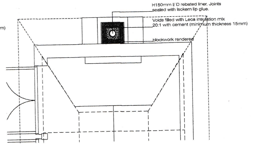
Plan above roof level
