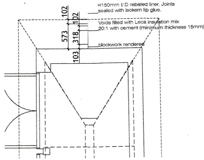
Plan above fire level
