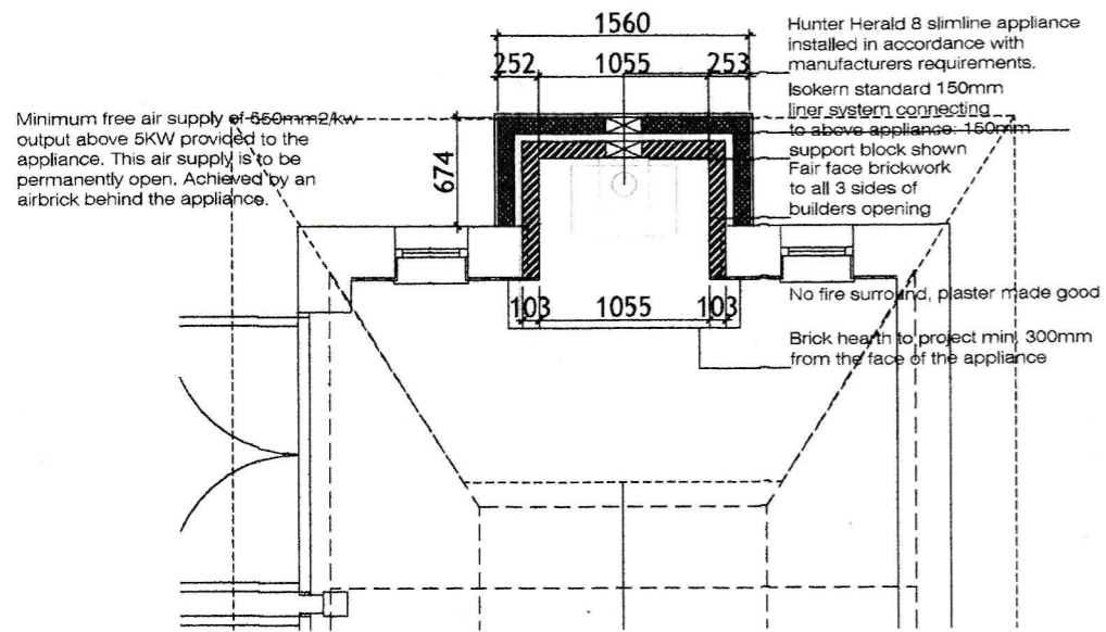
Plan at ground floor level
