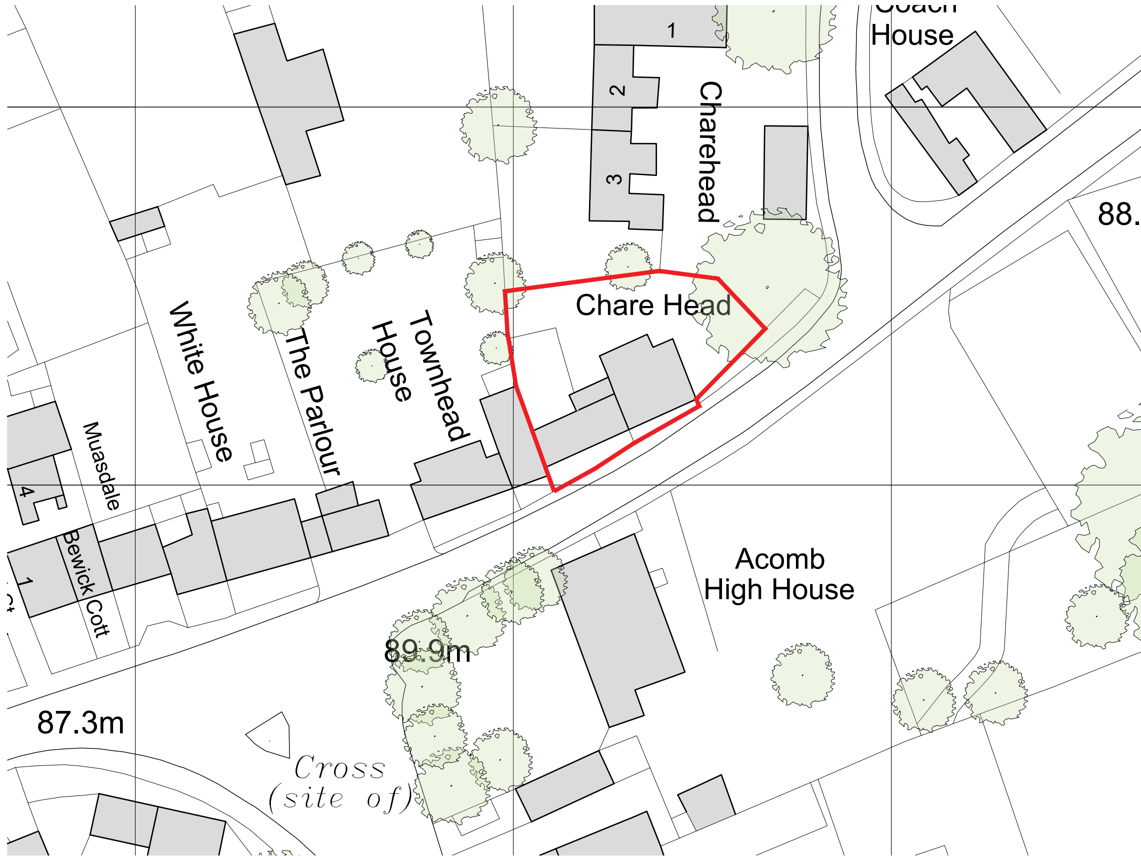
Proposed Site Plan Scale 1:500 @ A3
