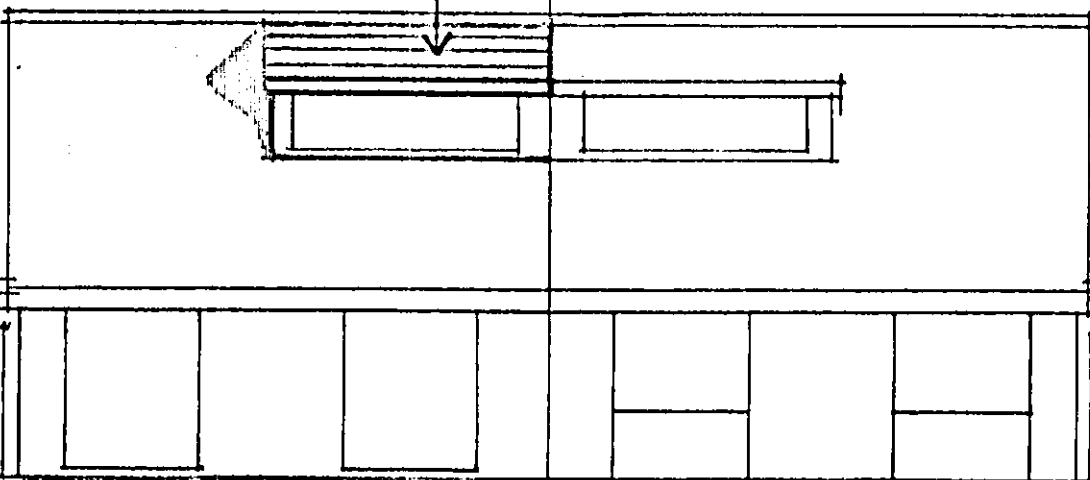
PROPOSED FRONT / EAST ELEVATION. 1/100
