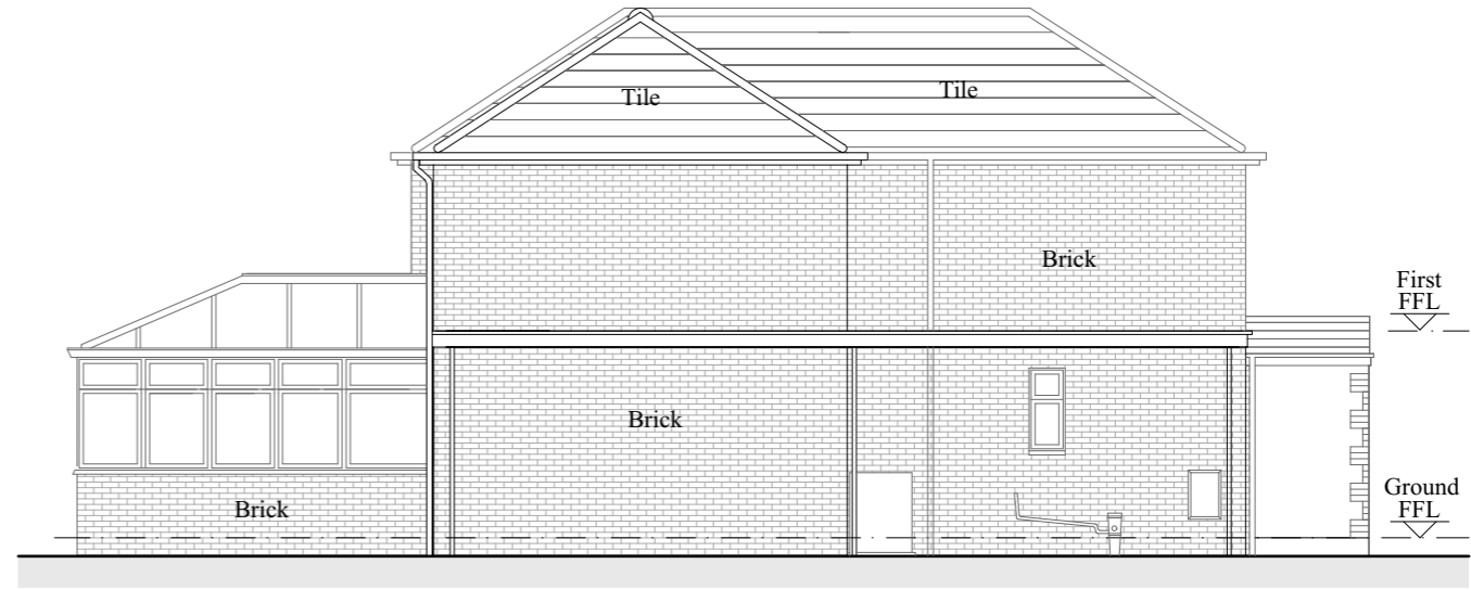
Existing Side 2 Elevation
