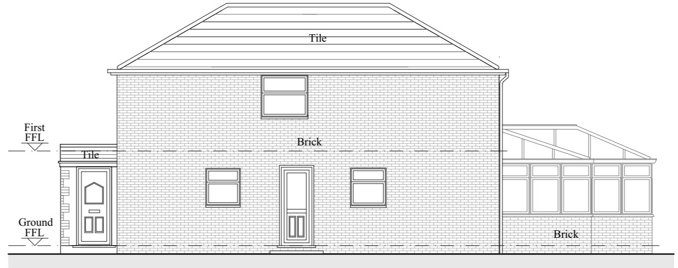
Existing Side 1 Elevation
