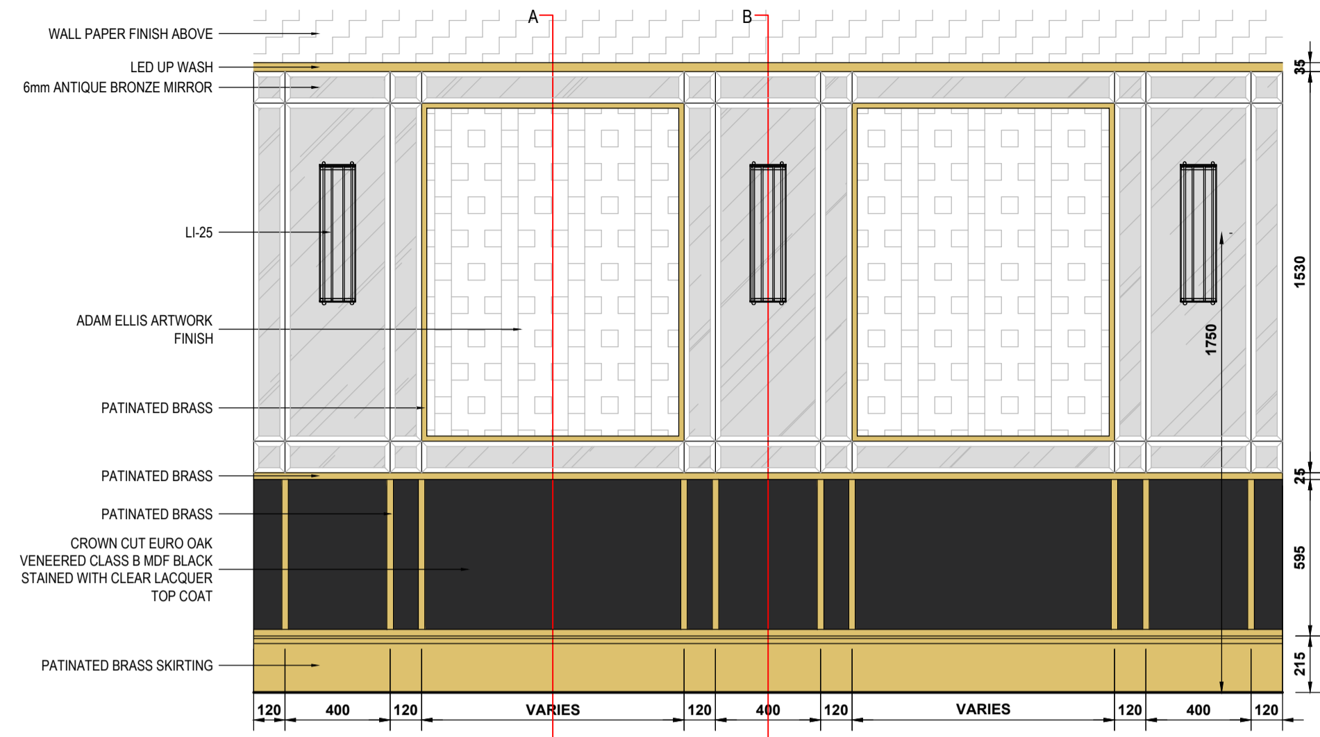
WALL PANELLING ARRANGEMENT @ 1:20
