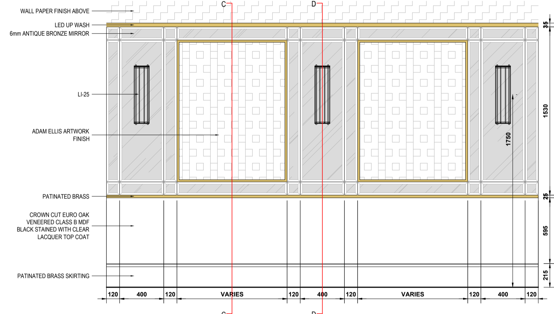
WALL PANELLING ARRANGEMENT WITH BANQUETTE @ 1:20
