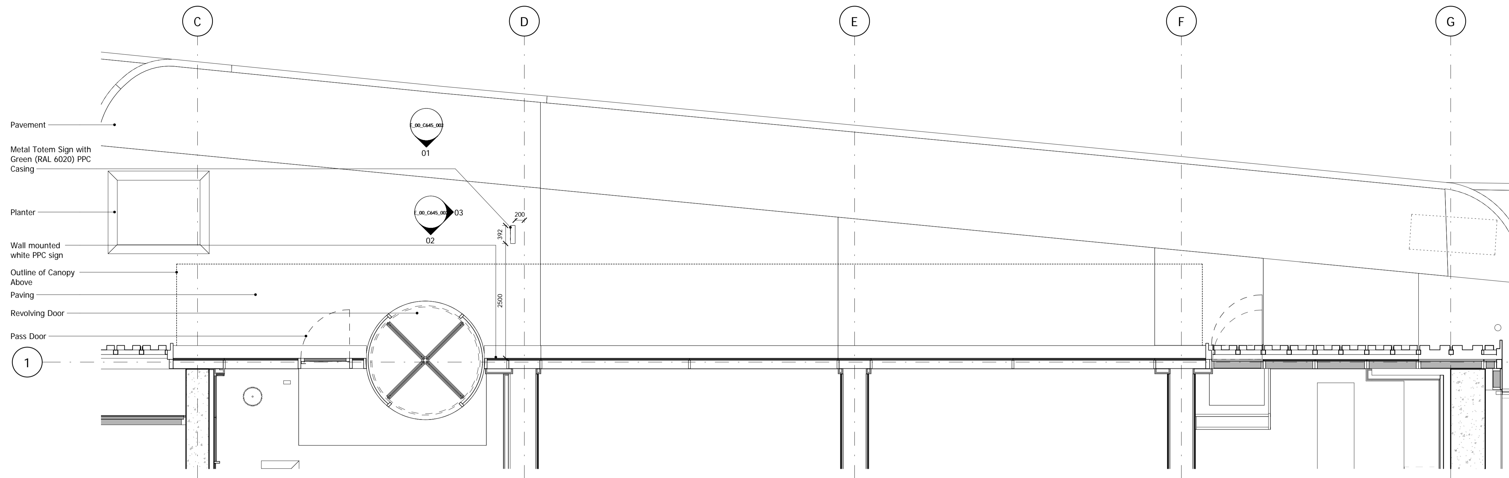
01 Planning Signage Location Plan - Ground 1 : 50
