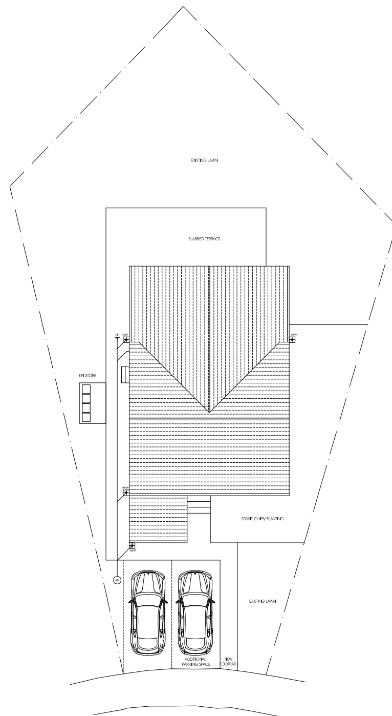
SITE PLAN AS PROPOSED
