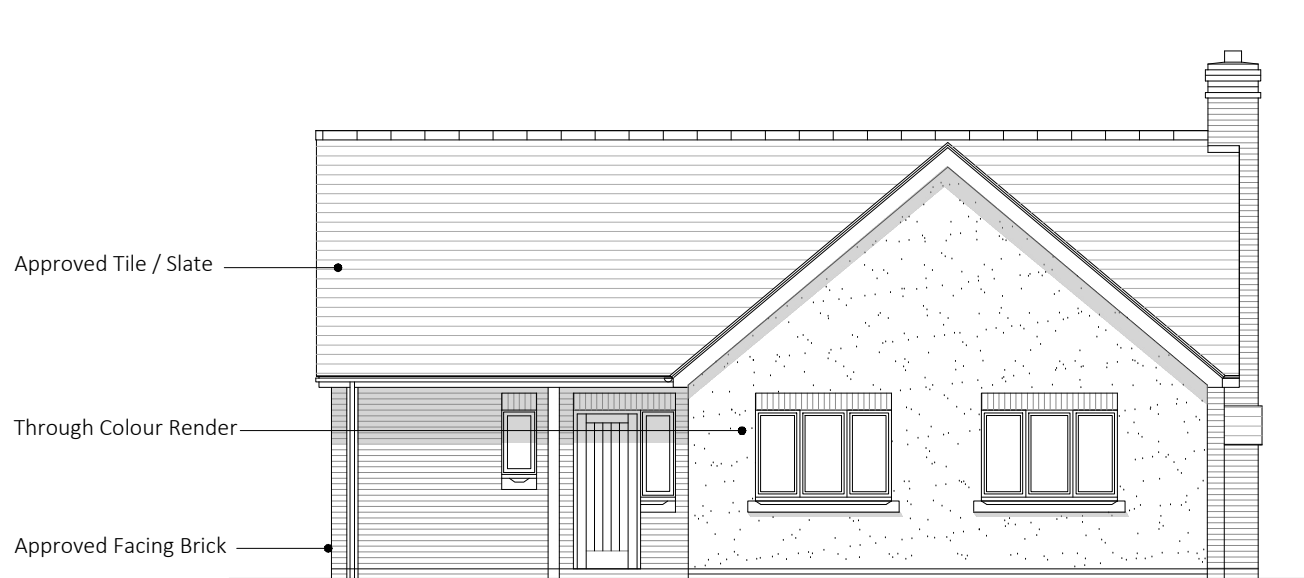
Front Elevation
