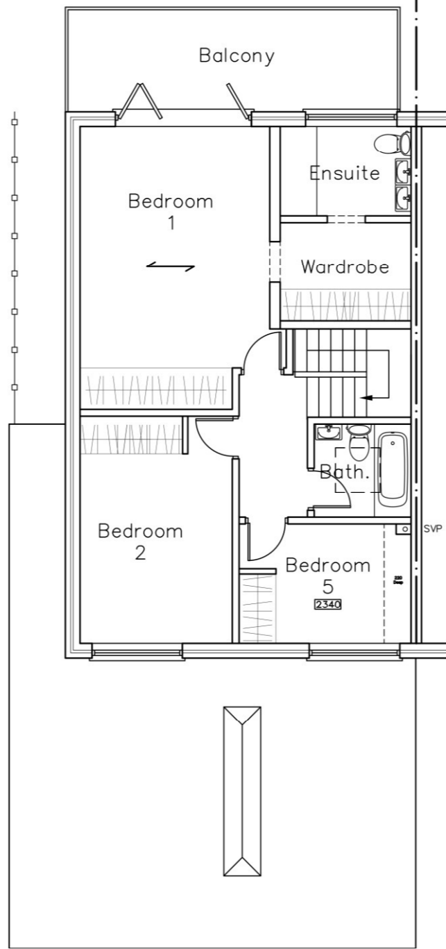
First Floor
