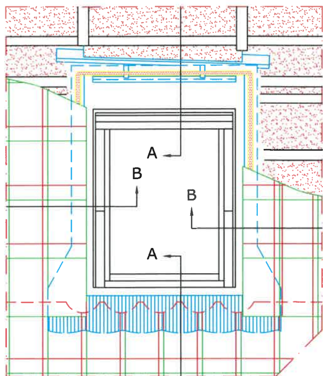
TYPICAL ELEVATION
