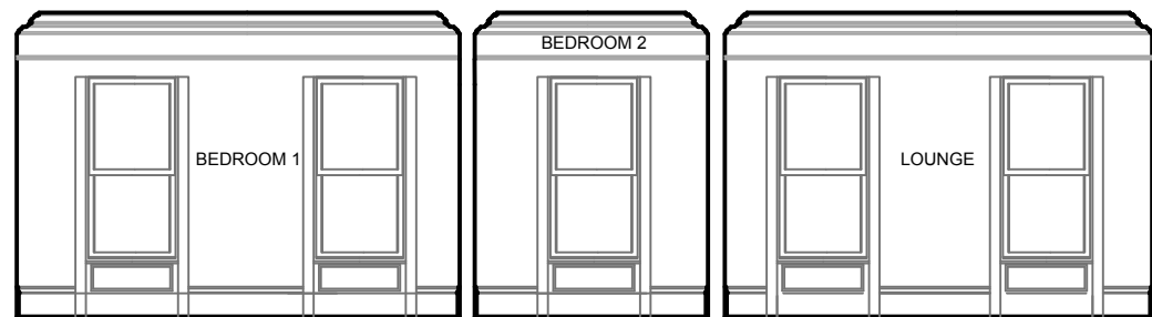
SECTION B-B AS EXISTING
