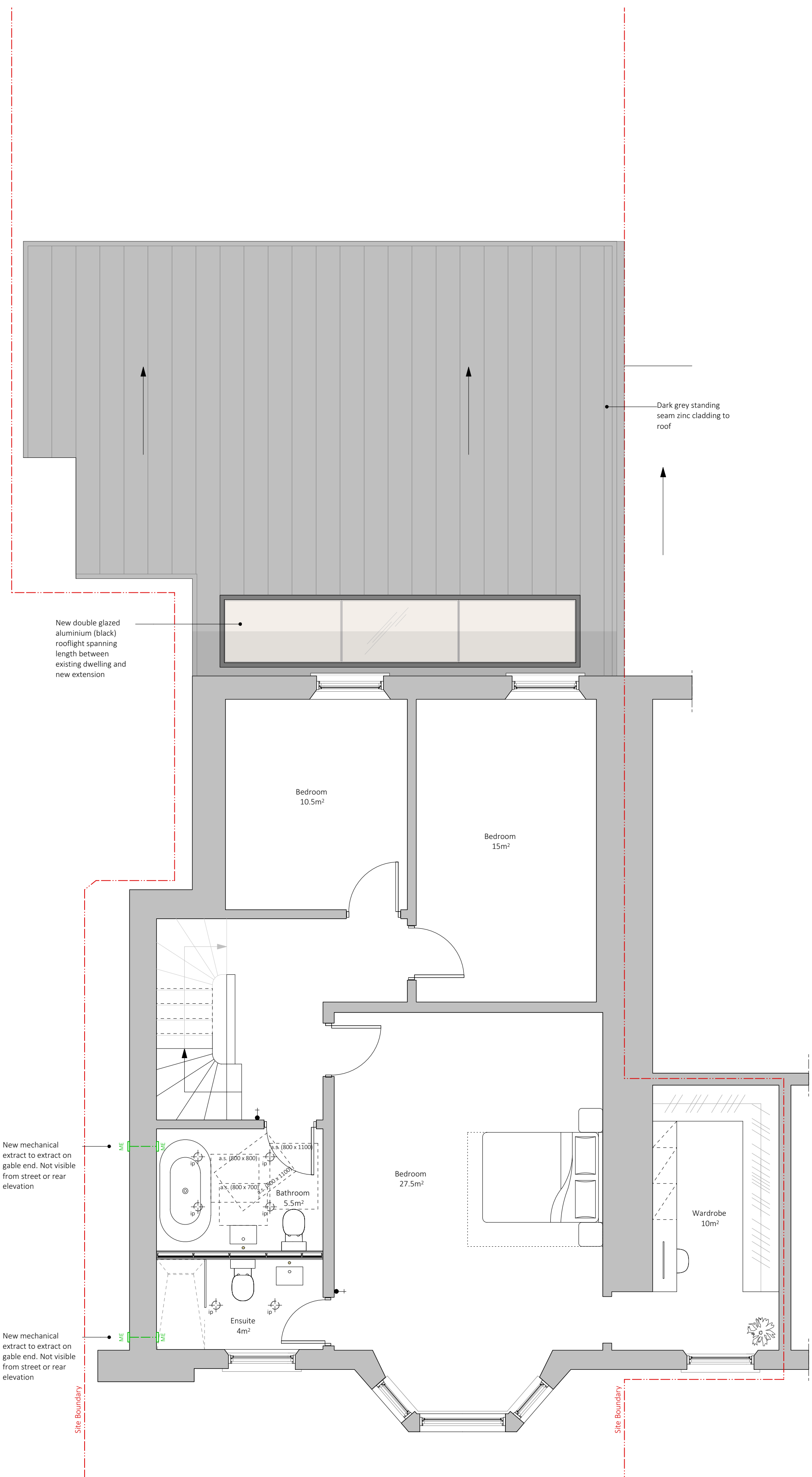
First Floor - as existing Scale 1:50
