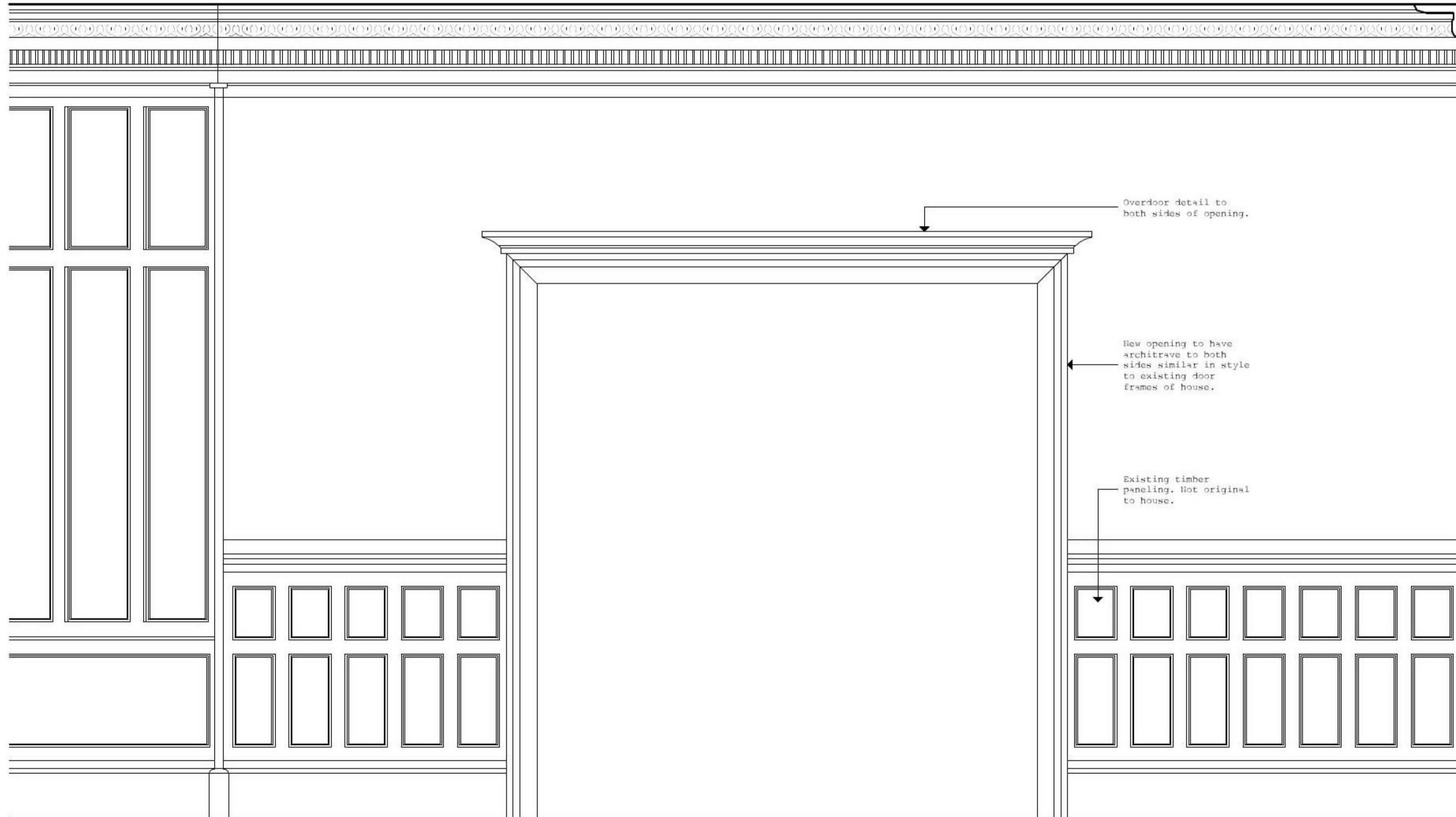
FL 01 - Dining Room Elevation - Proposed
