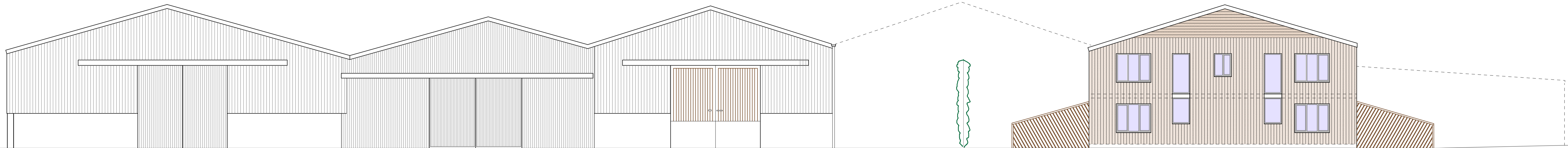
ROADSIDE ELEVATION
