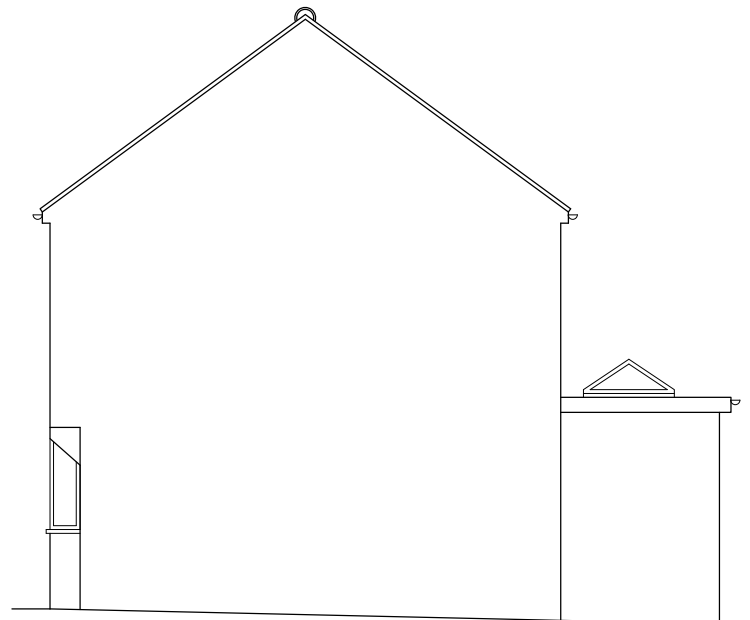
EXISTING SOUTH WEST ELEVATION
