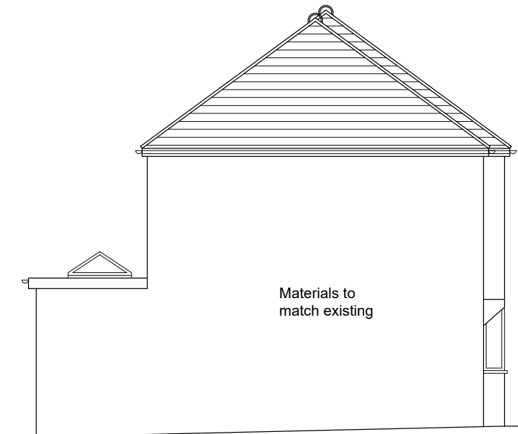
PROPOSED NORTH EAST ELEVATION
