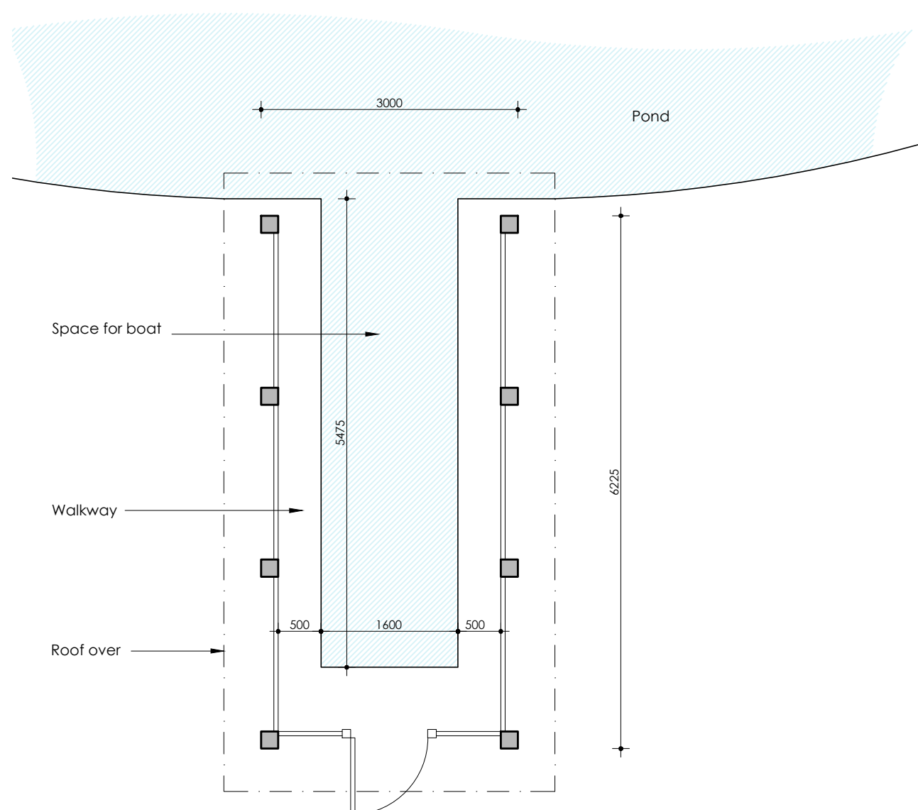
Floor Plan
