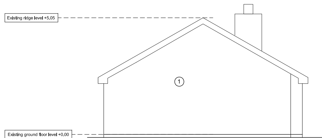
Existing side elevation (West)
