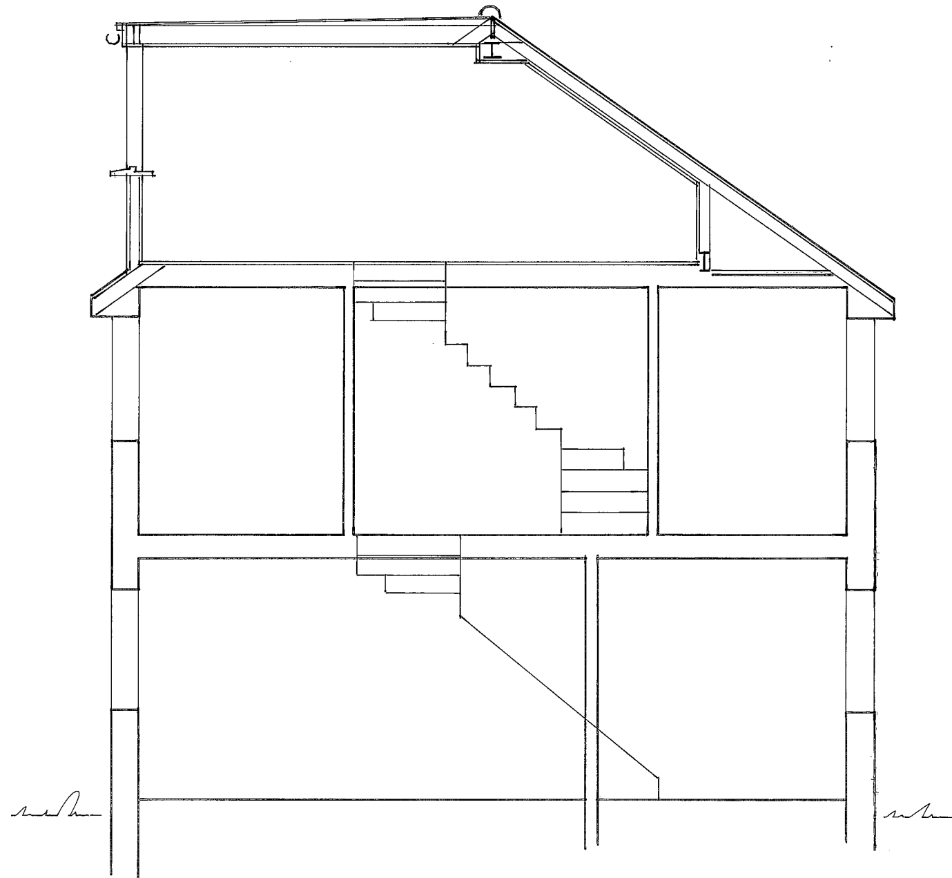
Dormer Cross-Section
