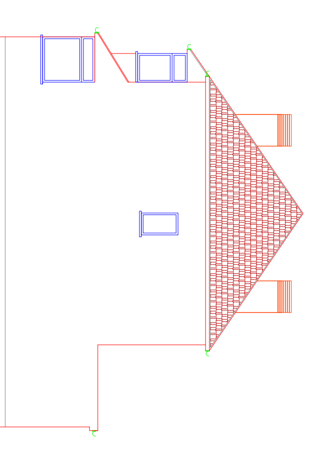
EXISTING RIGHT SIDE VIEW
