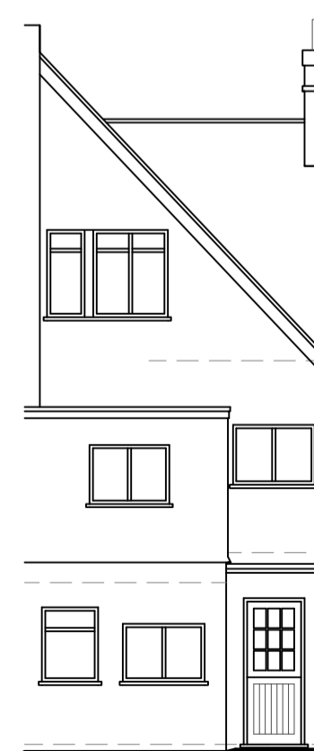
Rear elevation 1:100
