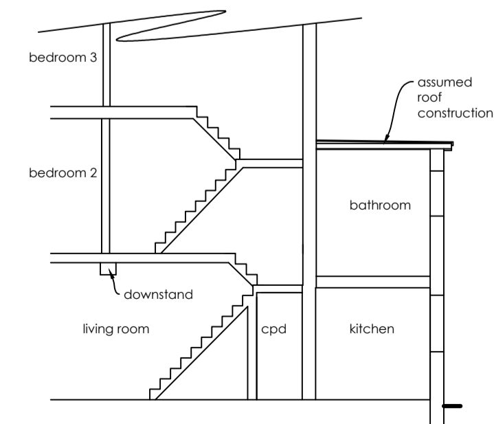
Section A - B 1:100
