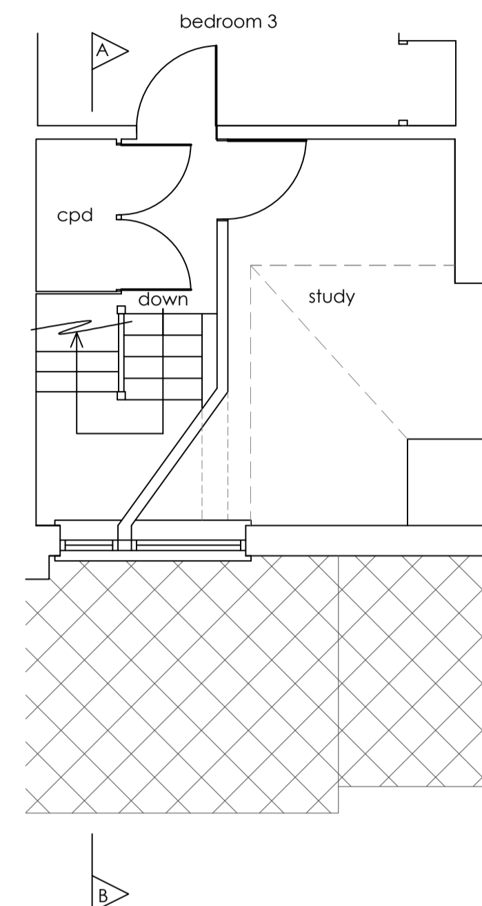
Second floor plan 1:50
