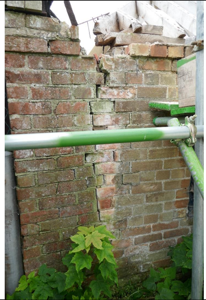
Example of cracking to the north elevation
