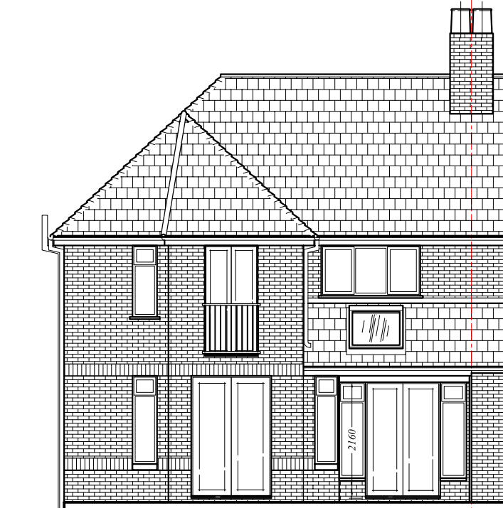
Rear Elevation
