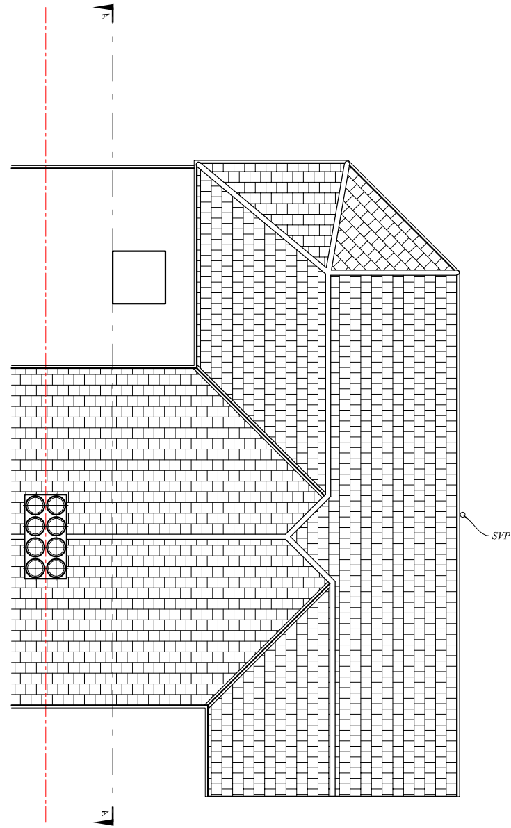
Roof Plan
