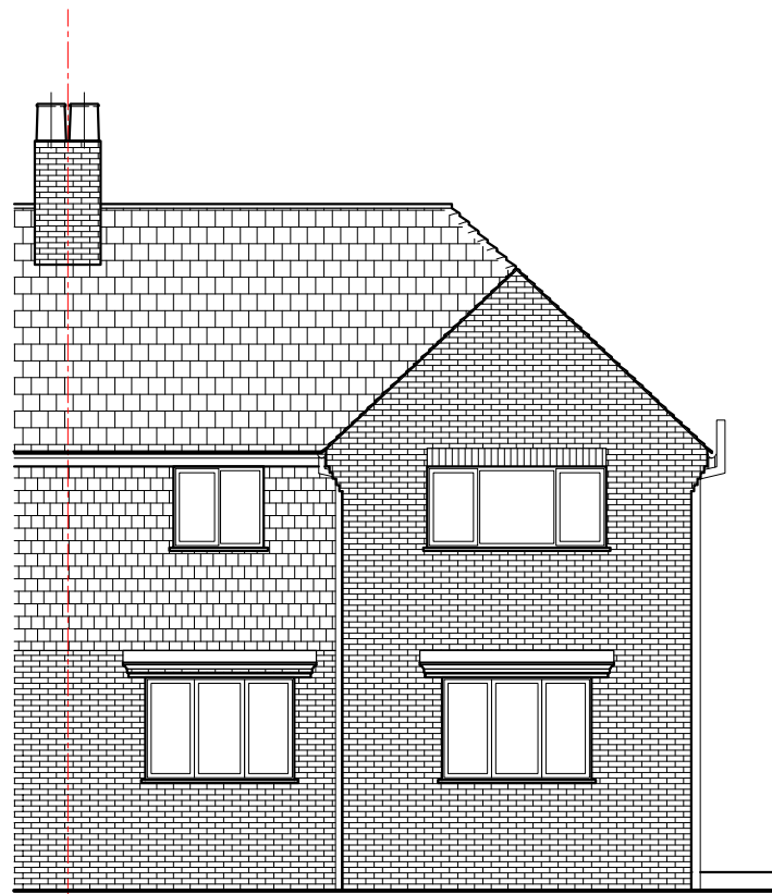
Front Elevation
