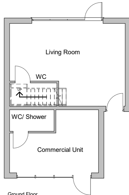
Ground Floor 1 : 100
