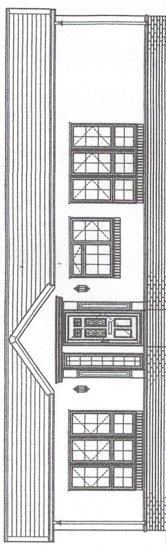
Nearside Elevation
