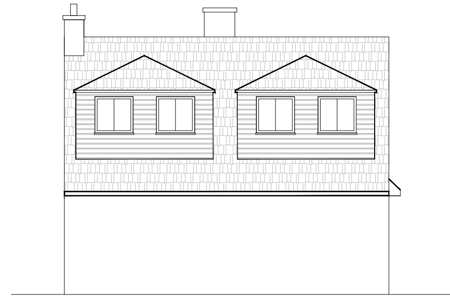
SOUTH ELEVATION AS PROPOSED
