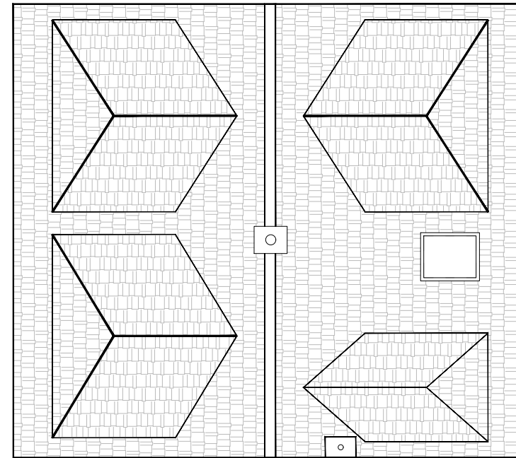
ROOF PLAN AS PROPOSED
