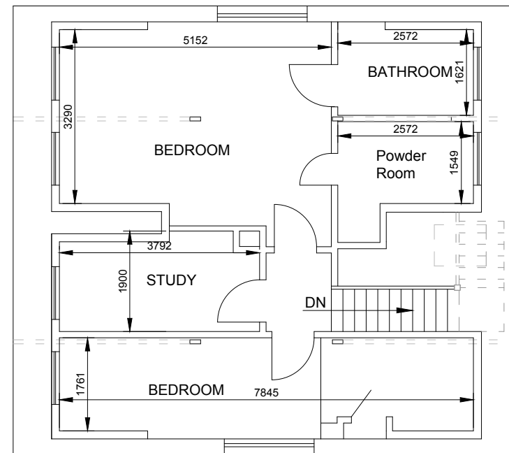
LOFT FLOOR PLAN AS PROPOSED
