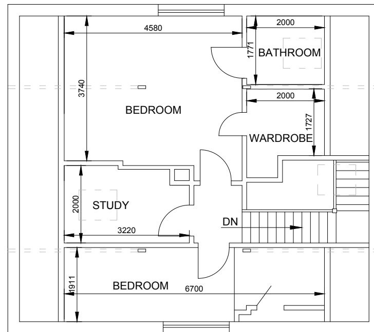
LOFT FLOOR PLAN AS EXISTING
