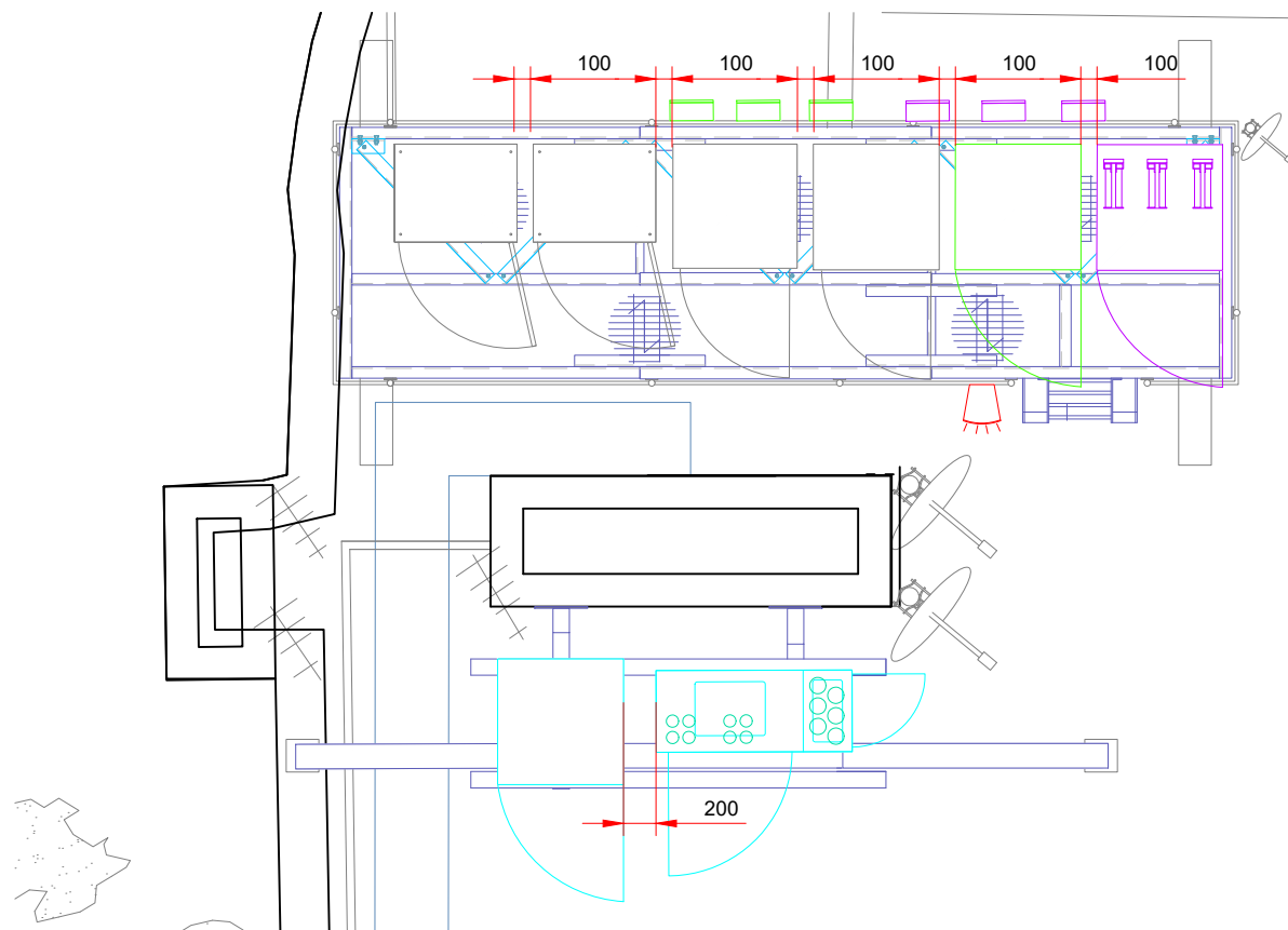
PROPOSED CABINET SET OUT DIMENSIONS
