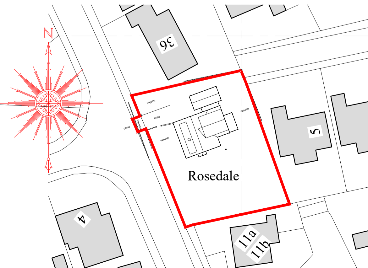
BLOCK PLAN (survey) (1:500) Ordnance Survey licence number 100012866
