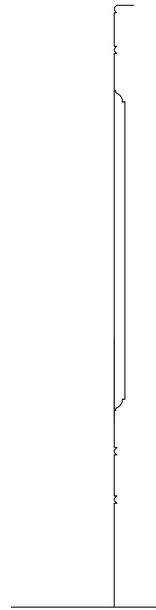
PART SECTION THROUGH THE PANELLING IN THE BEDROOM WINDOW REVEAL 1:5
