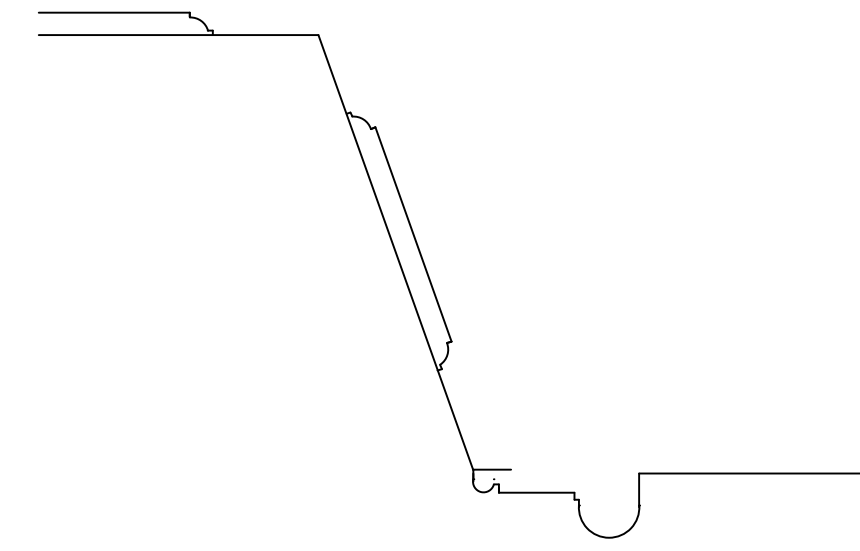
ARCHITRAVE AND PANELLING TO WINDOW REVEAL IN BATHROOM AND ENSUITE 1:5
