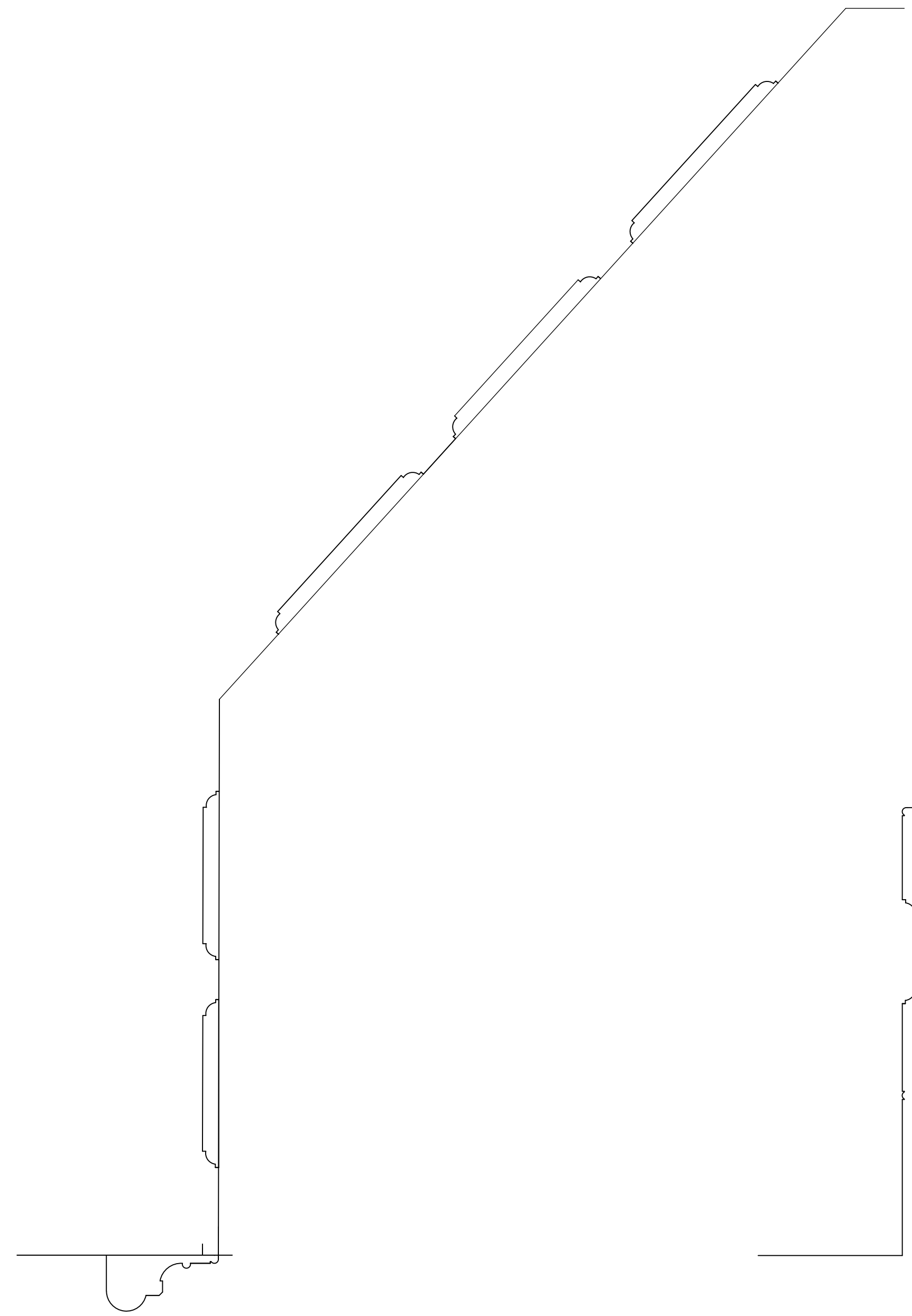
PART PLAN OF PANELLING TO BAY WINDOW IN THE DINING ROOM 1:5
