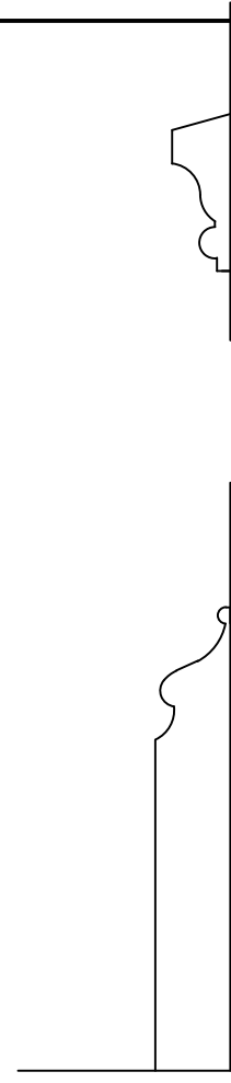
DINING ROOM DADO RAIL AND SKIRTING 1:5
