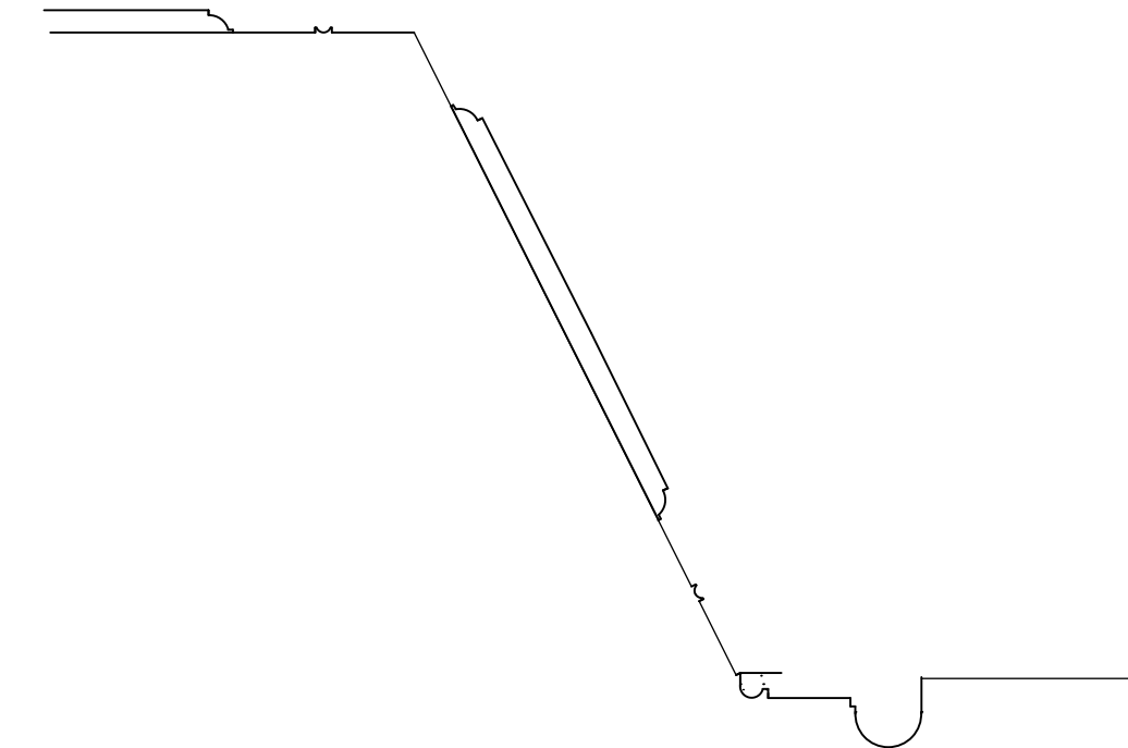
ARCHITRAVE AND PANELLING TO WINDOW REVEAL IN BEDROOM 1:5
