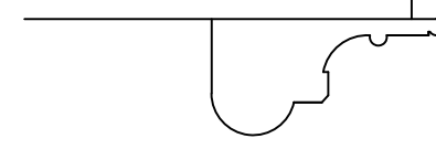
ARCHITRAVE TO BAY WINDOW IN DINING ROOM 1:5
