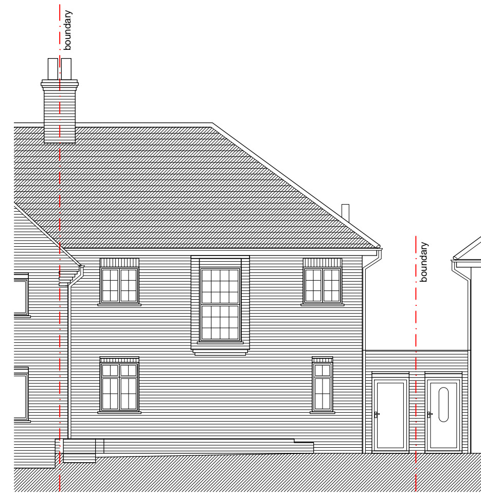
Front Elevation...
