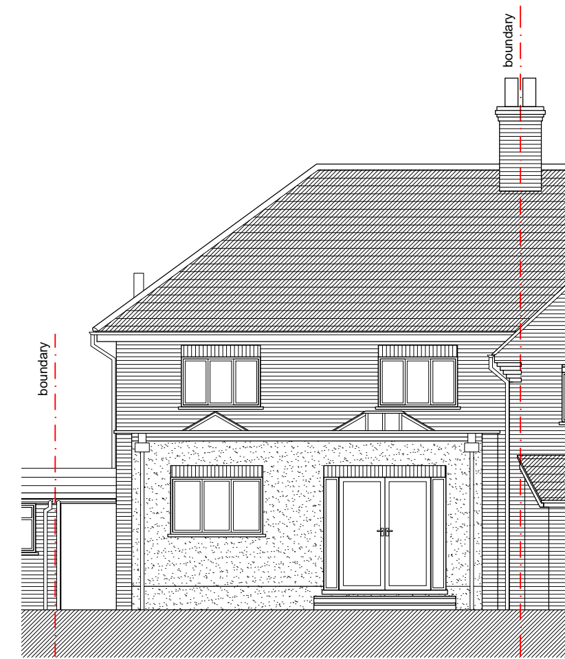
Rear Elevation...
