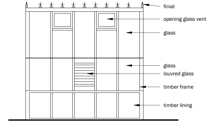
NW ELEVATION
