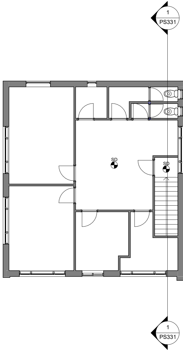
1 Existing First Floor layout 1 : 100
