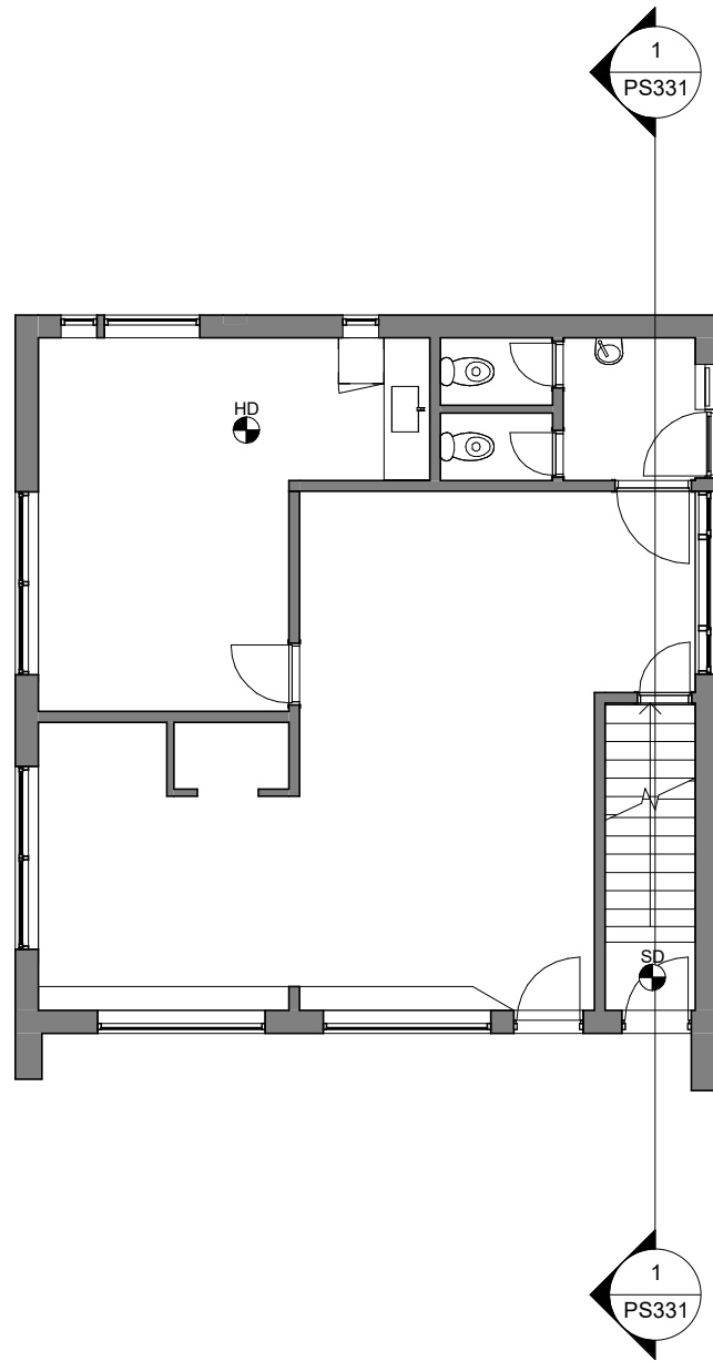
2 Existing Ground Floor layout 1 : 100
