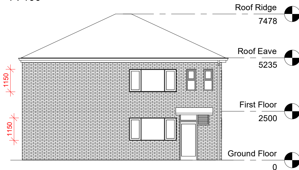
4 Proposed Right Elevation setout 1 : 100
