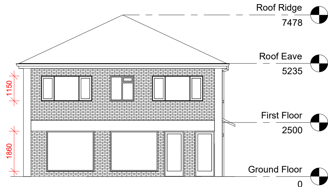
1 Proposed Front Elevation setout 1 : 100
