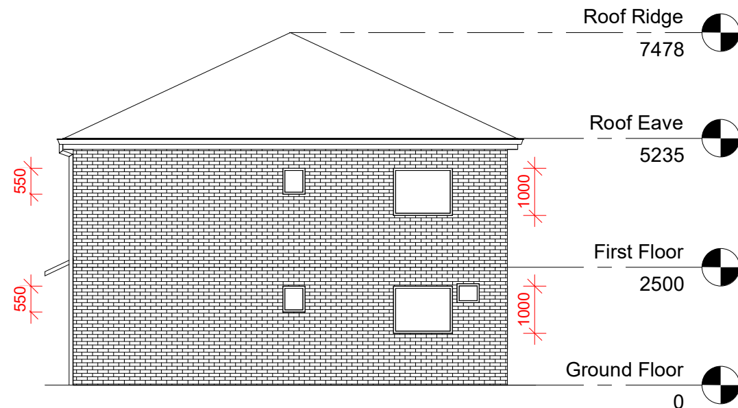
2 Proposed Rear Elevation setout 1 : 100
