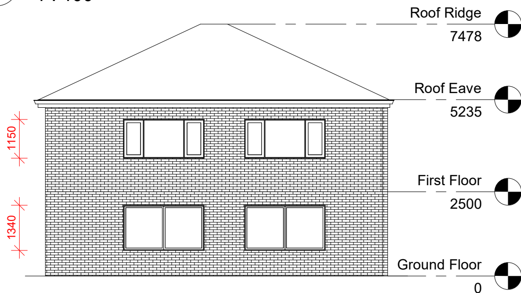
3 Proposed Left Elevation setout 1 : 100
