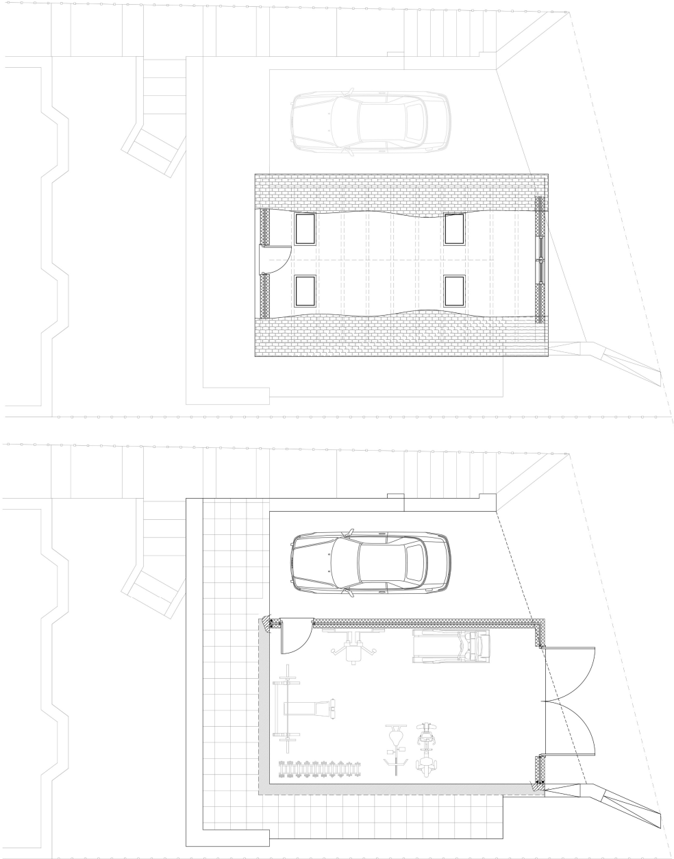
PROPOSED GARAGE PLAN 1 : 50
