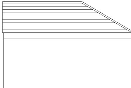
Rear/West Elevation
