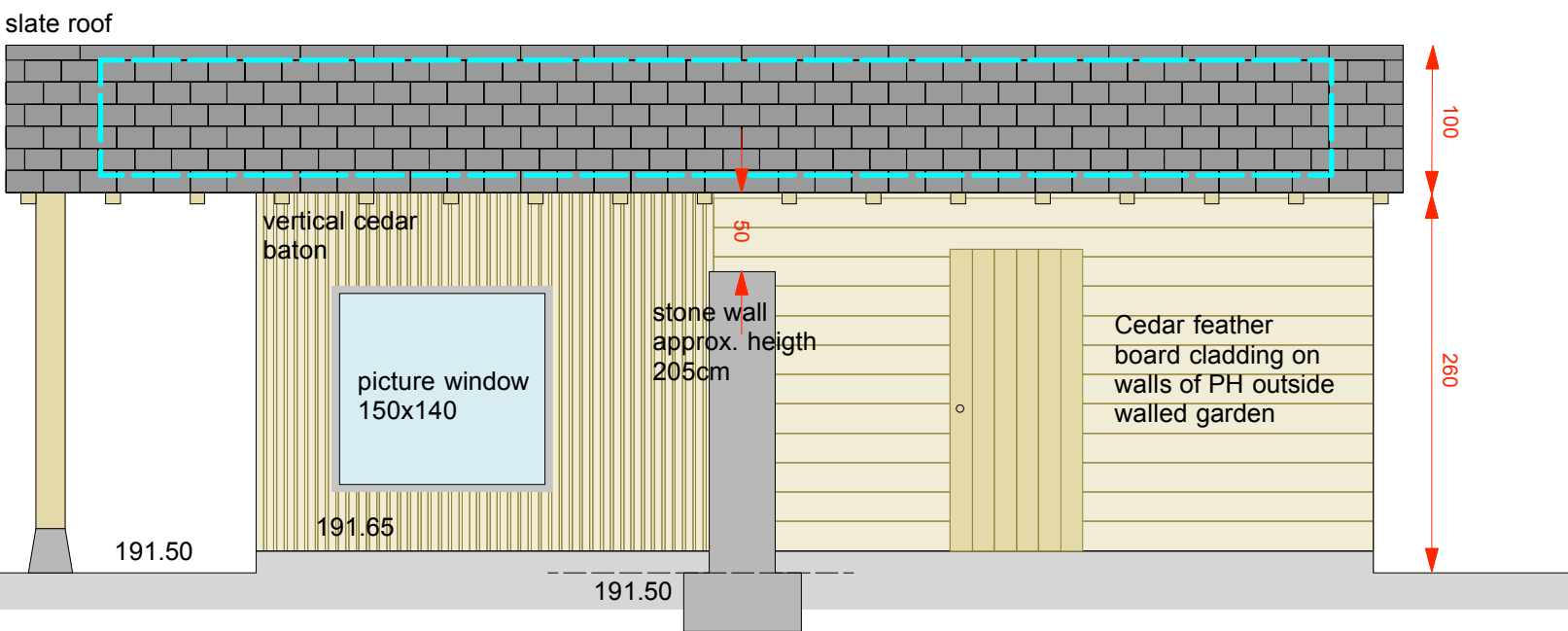
SOUTH ELEVATION
