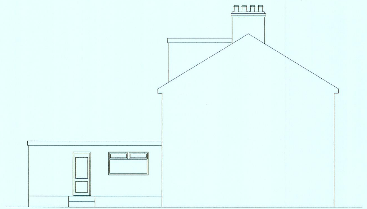
Proposed Side
