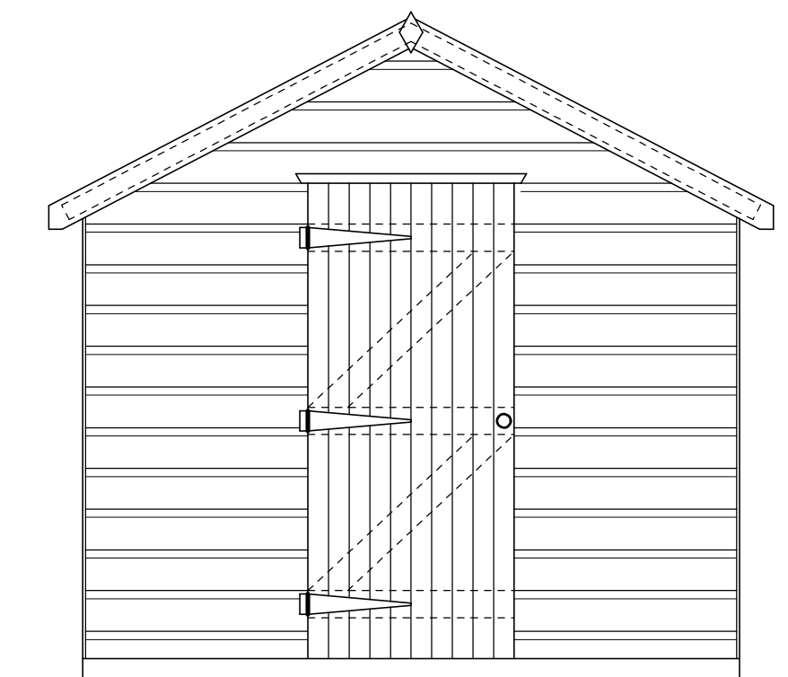
FRONT ELEVATION TO BUNGALOW
