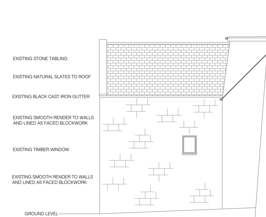
South-East Elevation 1:100
