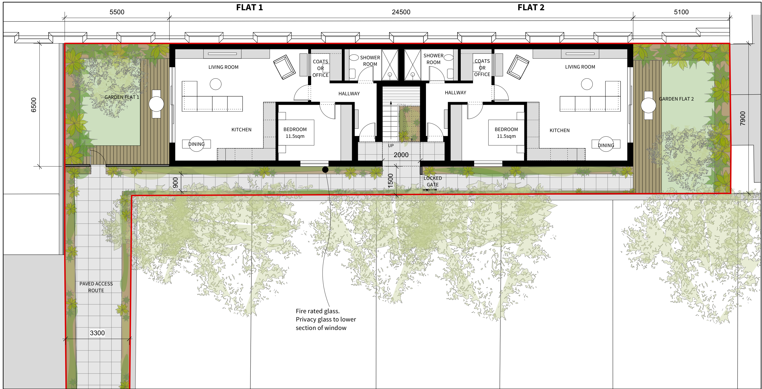
1 Proposed Ground Floor Scale: 1:100 2no - 2 Person Garden Flats Flat 1: 61sqm/ Garden: 35sqm Flat 2: 61sqm/ Garden: 57sqm
