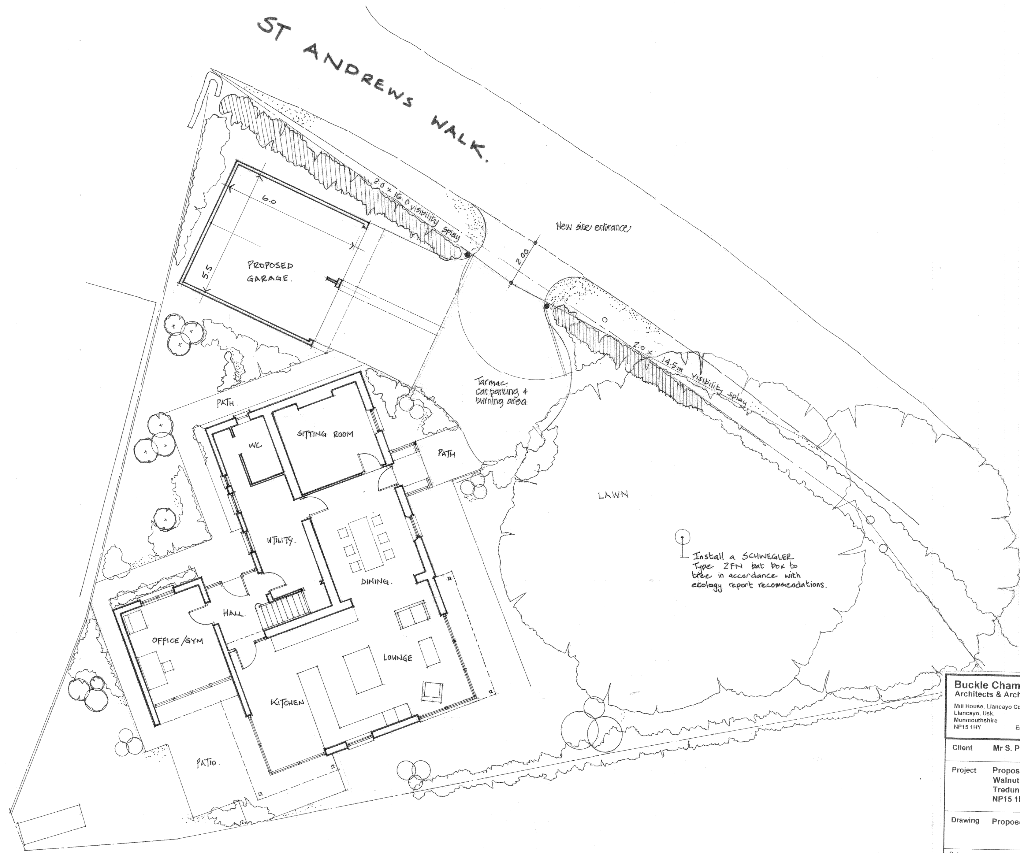
PROPOSED FLOOR /SITE BLOCK PLAN. (1:100)
