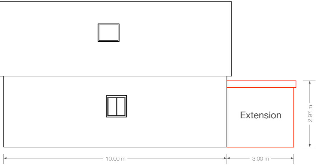
RH Side Elevation
