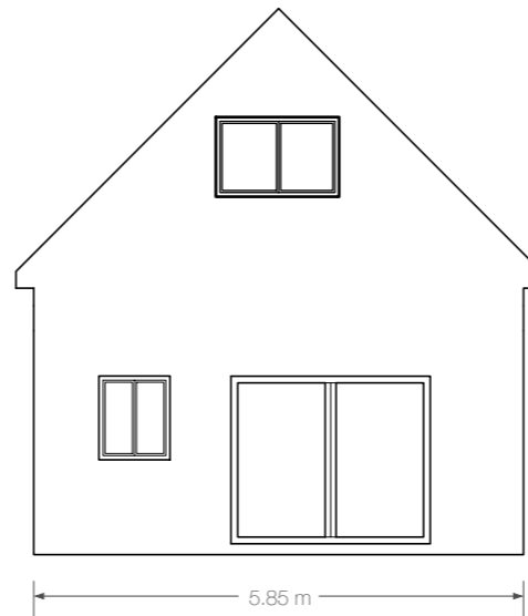
Rear Elevation
